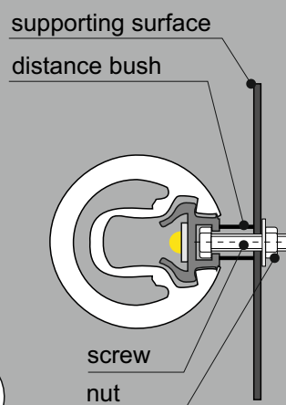
Wall mounting
